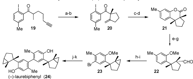
Scheme 1. Total Synthesis of (–)-Laurebiphenyl a
